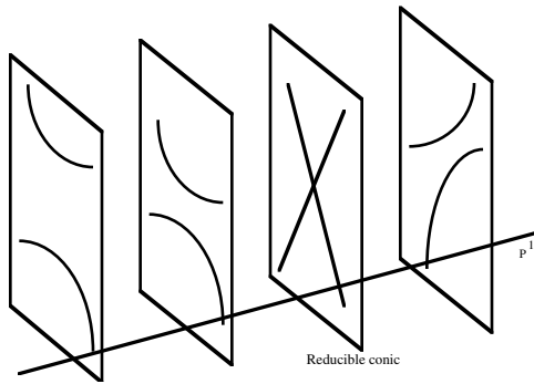
A Pencil of Conics Showing a Reducible Conic
